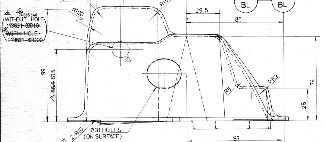
SECT. A-A
