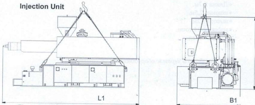
Figure 3-1 Side view of the machine being lifted using a wire rope connected to the frame
