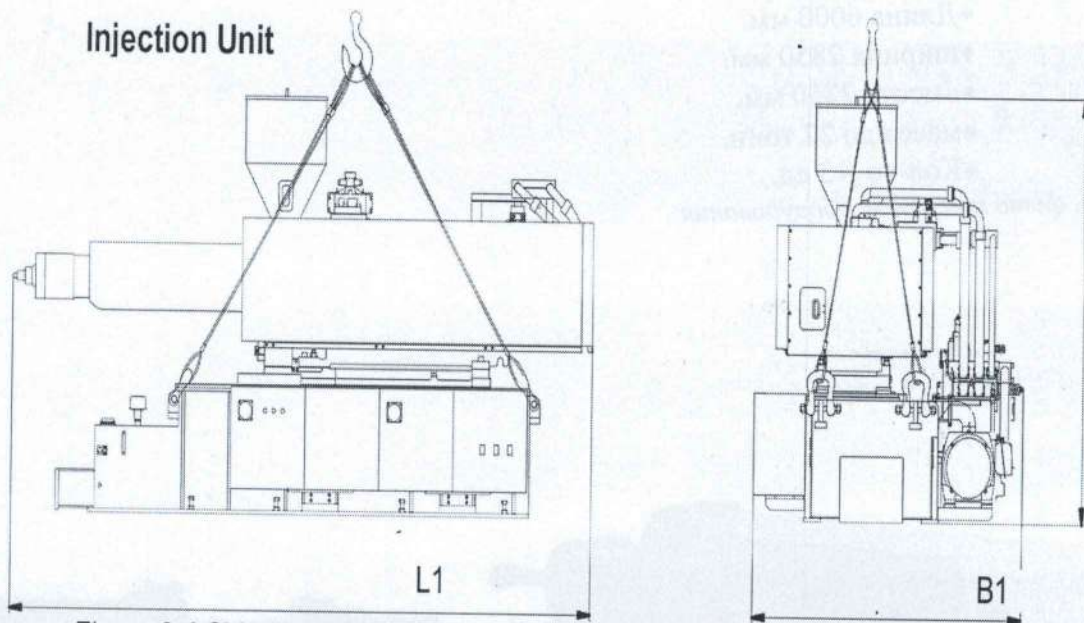
Figure 3-1 Side view of the machine being lifted using a wire rope connected to the frame
